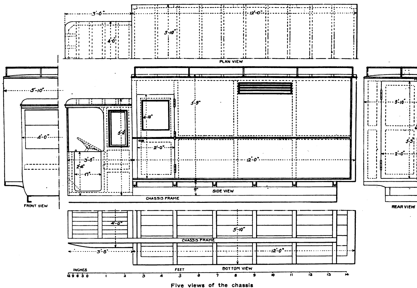
Five views of the chassis
